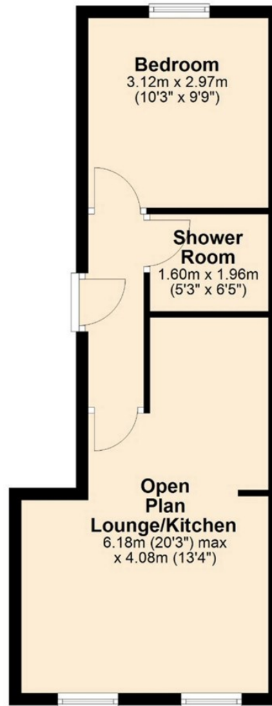
Floor Plan
