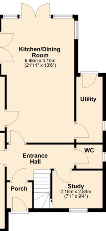
Ground Floor sq. metres (1026.5 sq. feet)
