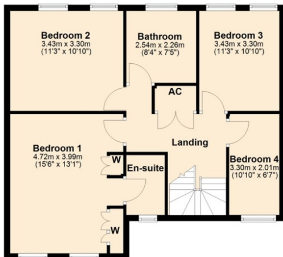
First Floor Approx. 69.8 sq. metres (750.8 sq. feet)
